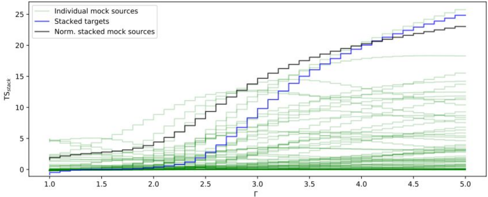
Figure from de Menezes et al. (Submitted to MNRAS on June 2021)
