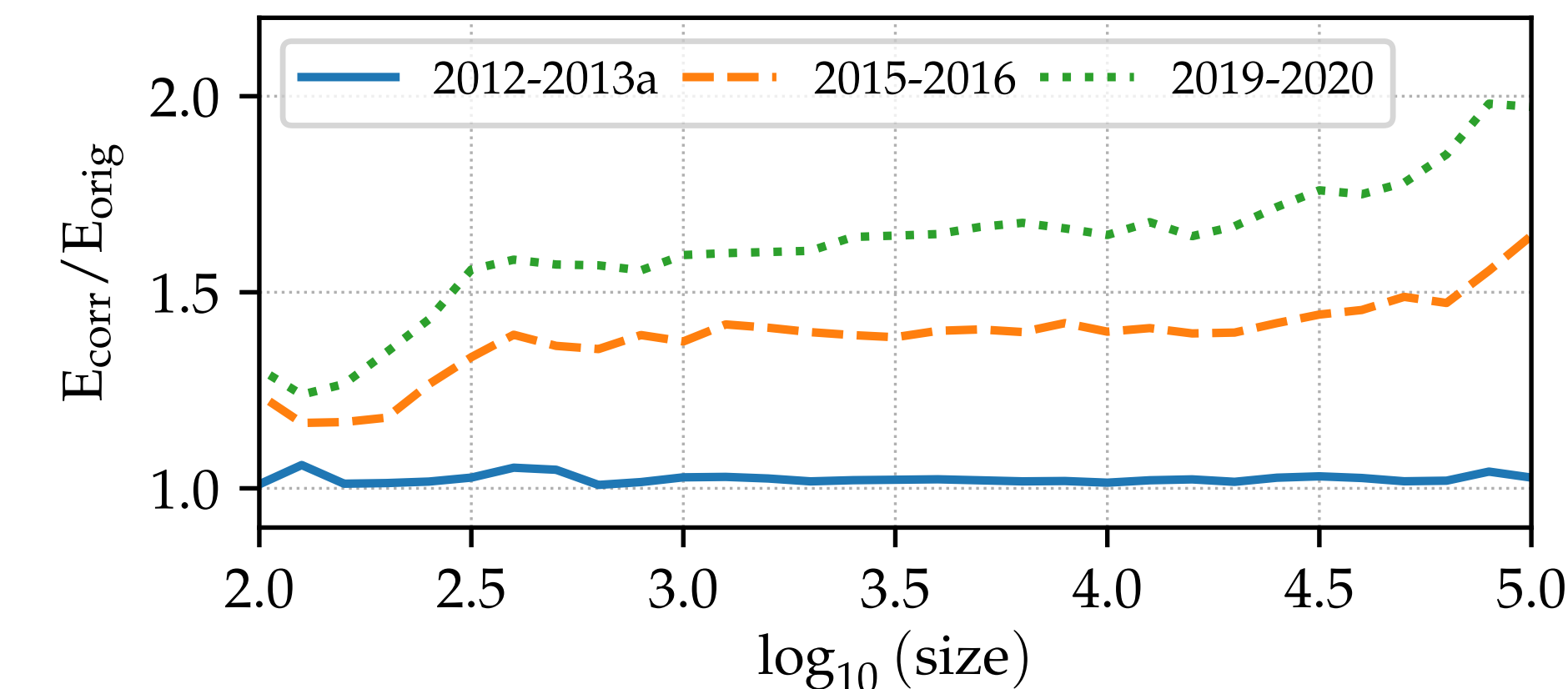
Figure 2: Ratio of throughput-calibrated E_{corr} to uncalibrated E_{orig} reconstructed energies (for telescope T1) as a function of size of the images, fixing all the other parameters involved in the construction of the tables (noise, shower distance, zenith, etc). Three different IRF periods are shown.
