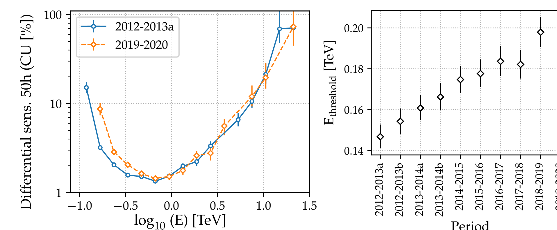
Figure 3: left: Differential sensitivity. right: Energy threshold. They were obtained using Crab Nebula data and for a typical set of analysis cuts.
