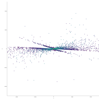
(b) Counter-clockwise helicity
