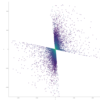
(c) Zero helicity
