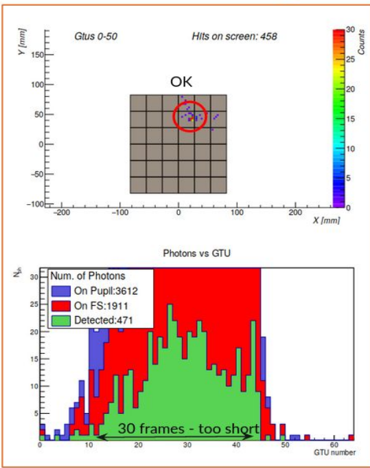
Left: Mini-EUSO event detected over the ocean, off the coast of Sri Lanka . Center and Right: EAS simulated through ESAF with different energy and zenith angle. The simulation with Z = 50^\circ and energy 5 \times 10^{21} eV produce a footprint on the focal plane similar to the event but the lightcurve is too short, while the event at Z = 80^\circ and energy 2 \times 10^{22} eV correctly reproduces the lightcurve but has a different shape.
