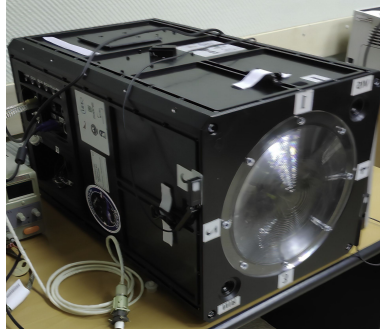
Exterior view of Mini-EUSO. One of the two Fresnel lenses is clearly visible
