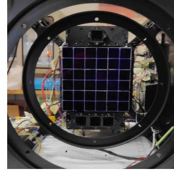
Focal plane of Mini-EUSO. The focal plane is made of an array of 36 MAPMTs, for a total of 2304 pixels (48x48)
