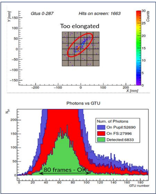
Left: Mini-EUSO event detected over the ocean, off the coast of Sri Lanka . Center and Right: EAS simulated through ESAF with different energy and zenith angle. The simulation with Z = 50^\circ and energy 5 \times 10^{21} eV produce a footprint on the focal plane similar to the event but the lightcurve is too short, while the event at Z = 80^\circ and energy 2 \times 10^{22} eV correctly reproduces the lightcurve but has a different shape.
