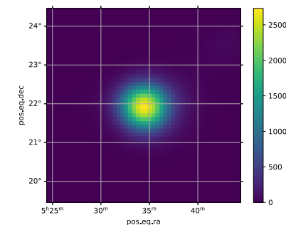
Test Statistic (TS) map
