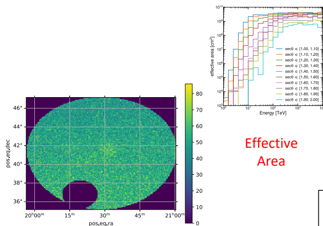
Fit region around Cygnus Cocoon
