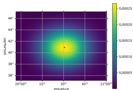
Spatial model of Cygnus Cocoon with a Gaussian width 2.13^\circ
