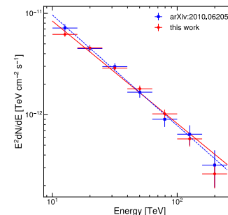
Spectral Energy Distribution (SED)
