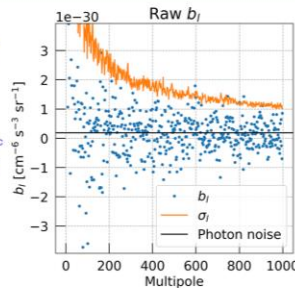
Diagonal bispectrum coefficients in the 26.5 to 64.7 GeV energy range with 1-sigma error and photon noise estimates.
