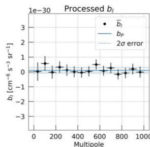
The diagonal coefficients after the application of binning. Blue line shows the obtained reduced bispectrum amplitude due to point sources and the 2-sigma confidence interval.
