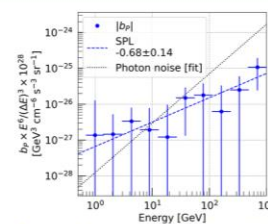
Bispectrum amplitude energy spectrum showing absolute values of obtained bispectrum amplitudes and best-fit power law model.
